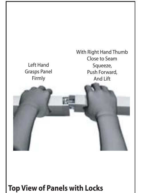
Top View of Panels with Locks The first level of components contain panel locks that are located at the top of the panel for extra stability and seamless connection. When disassembling panels twist top connection slightly and lift right panel upward.
